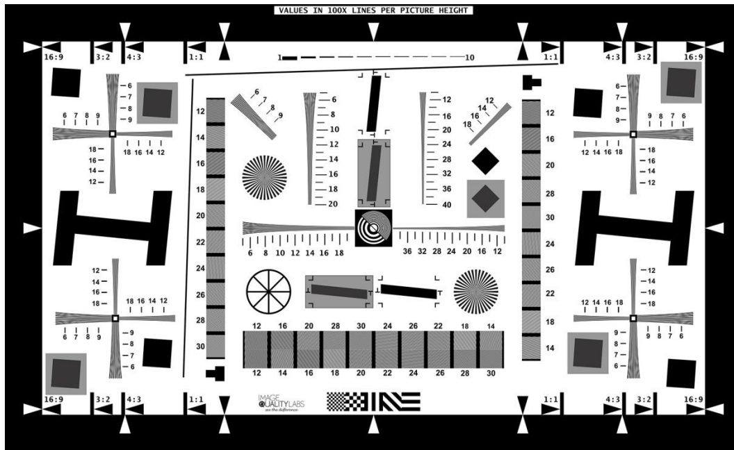
ISO 12233 Chart
